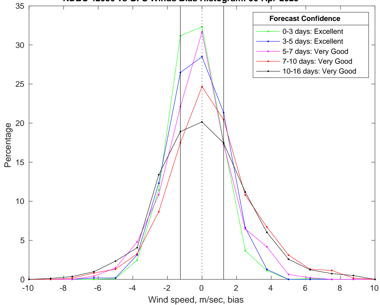
NDBC 42036 vs GFS Winds Bias Histogram: 30-Apr-2025
