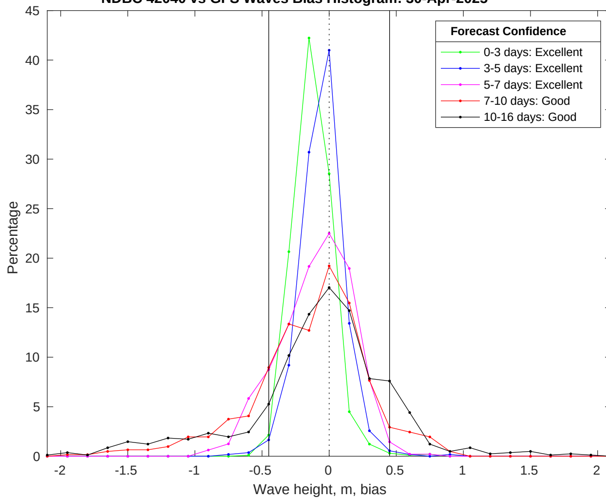
NDBC 42040 vs GFS Waves Bias Histogram: 30-Apr-2025
