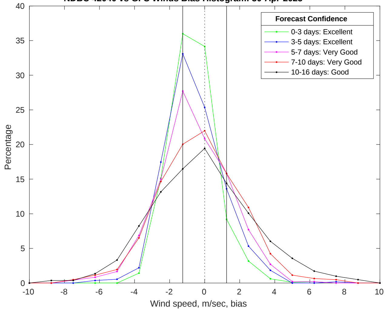
NDBC 42040 vs GFS Winds Bias Histogram: 30-Apr-2025
