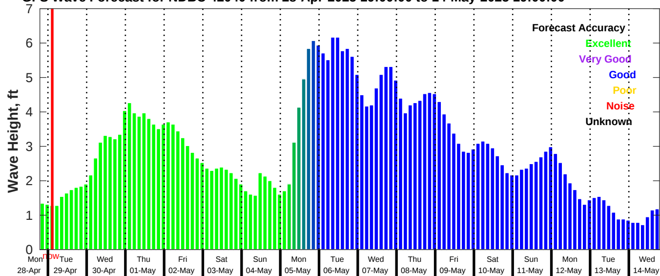
GFS Wave Forecast for NDBC 42040 from 28-Apr-2025 19:00:00 to 14-May-2025 19:00:00
