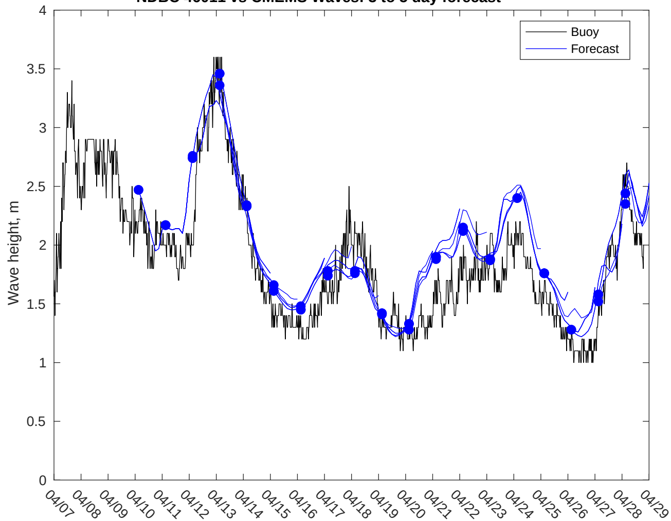
NDBC 46011 vs CMEMS Waves: 3 to 5 day forecast
