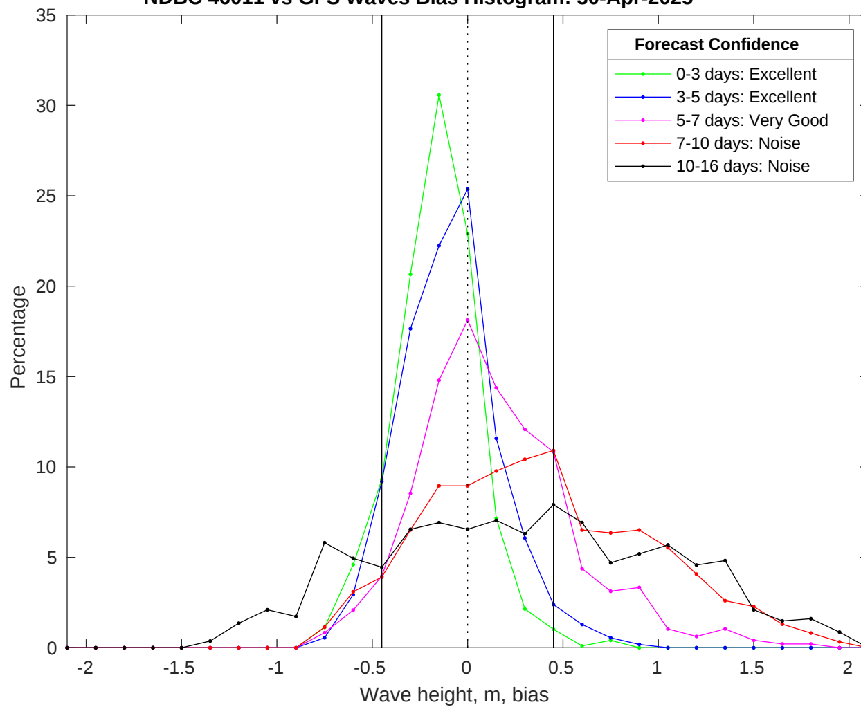
NDBC 46011 vs GFS Waves Bias Histogram: 30-Apr-2025
