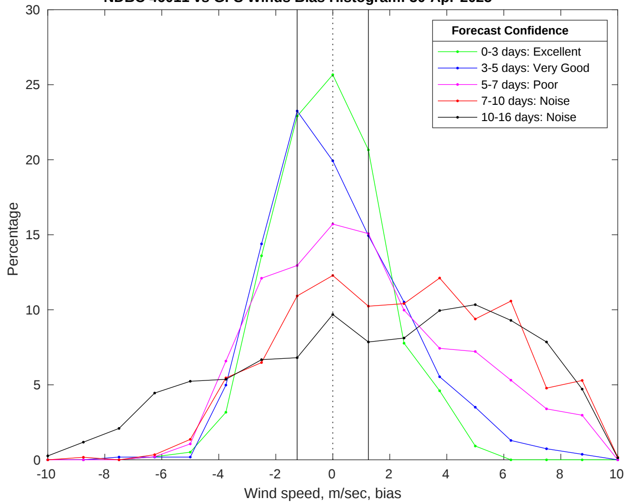
NDBC 46011 vs GFS Winds Bias Histogram: 30-Apr-2025
