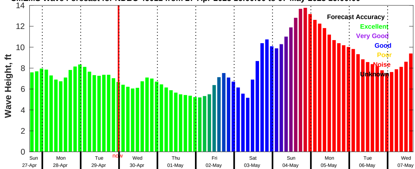
CMEMS Wave Forecast for NDBC 46011 from 27-Apr-2025 16:00:00 to 07-May-2025 16:00:00
