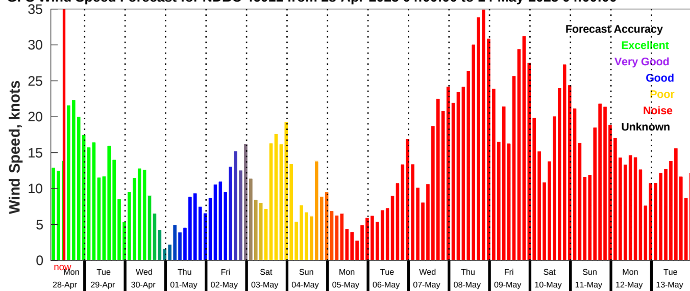
GFS Wind Speed Forecast for NDBC 46011 from 28-Apr-2025 04:00:00 to 14-May-2025 04:00:00
