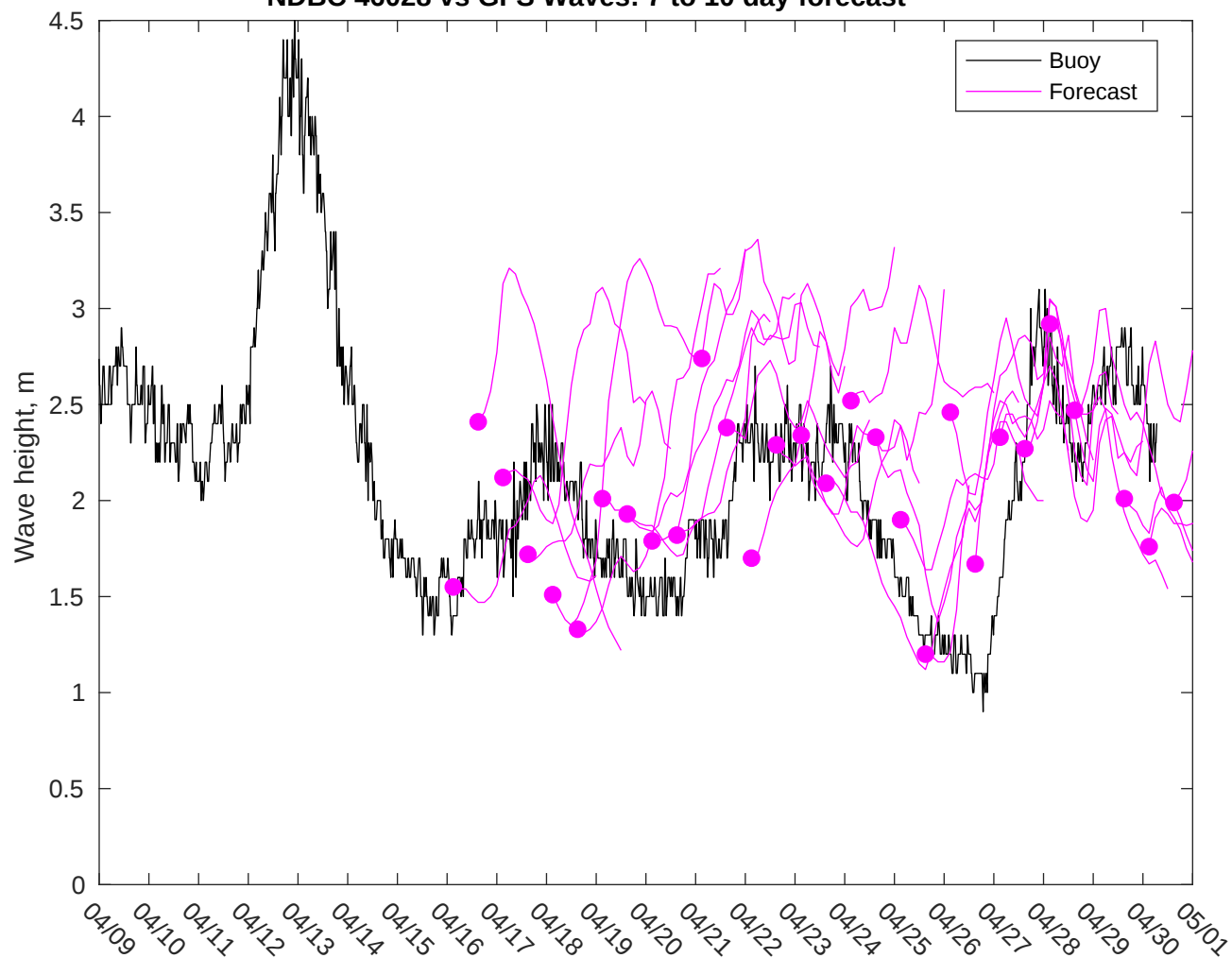
NDBC 46028 vs GFS Waves: 7 to 10 day forecast
