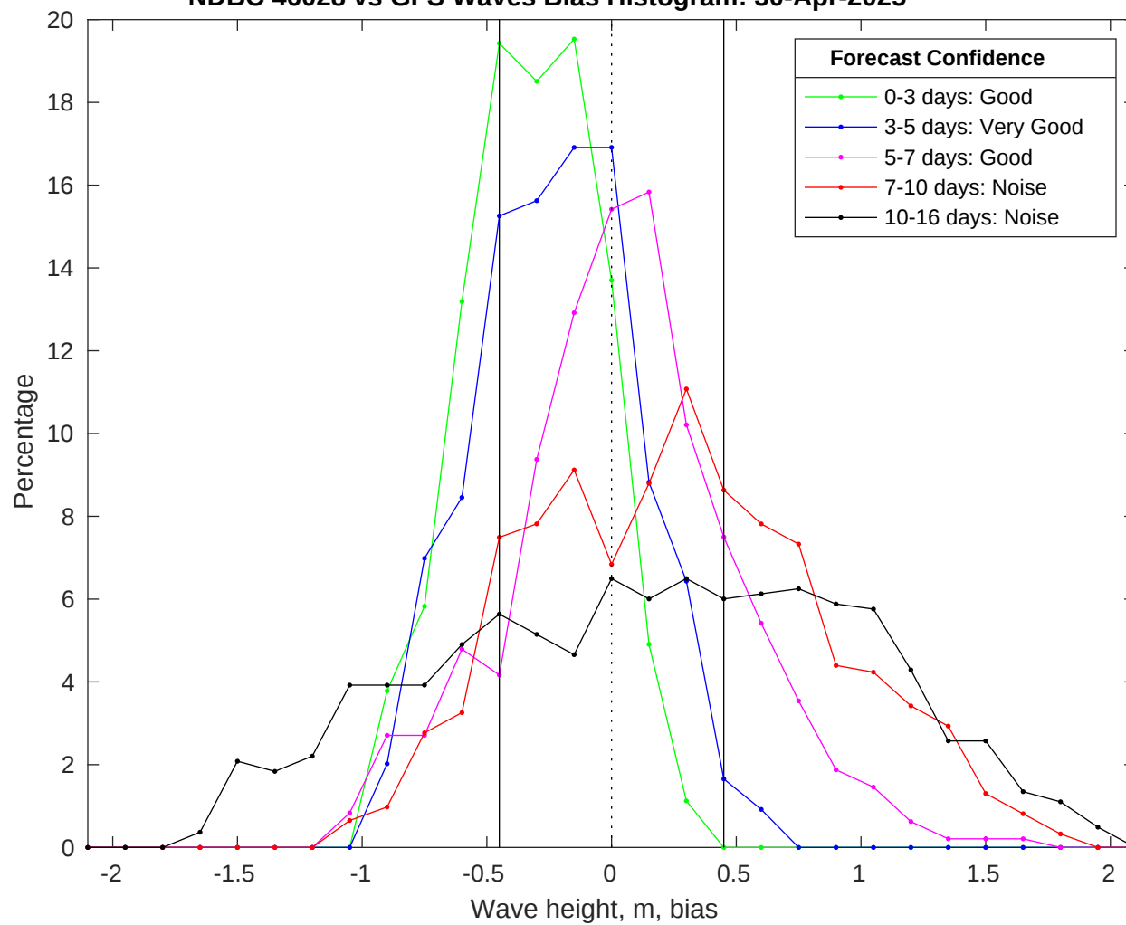
NDBC 46028 vs GFS Waves Bias Histogram: 30-Apr-2025
