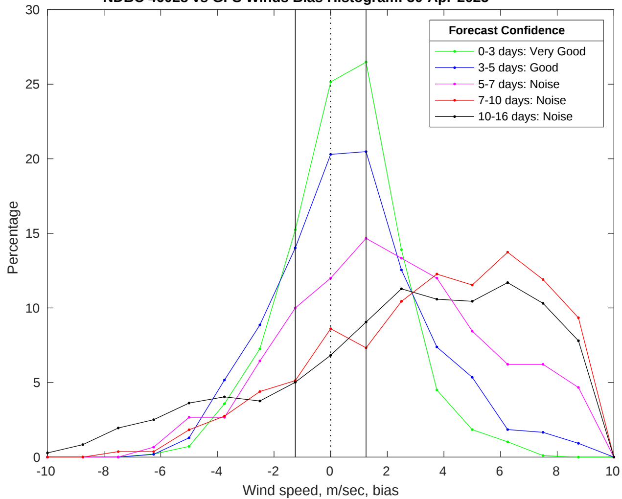
NDBC 46028 vs GFS Winds Bias Histogram: 30-Apr-2025
