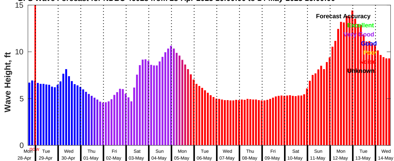
GFS Wave Forecast for NDBC 46028 from 28-Apr-2025 16:00:00 to 14-May-2025 16:00:00
