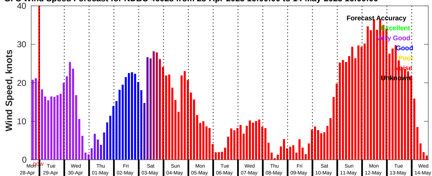
GFS Wind Speed Forecast for NDBC 46028 from 28-Apr-2025 16:00:00 to 14-May-2025 16:00:00
