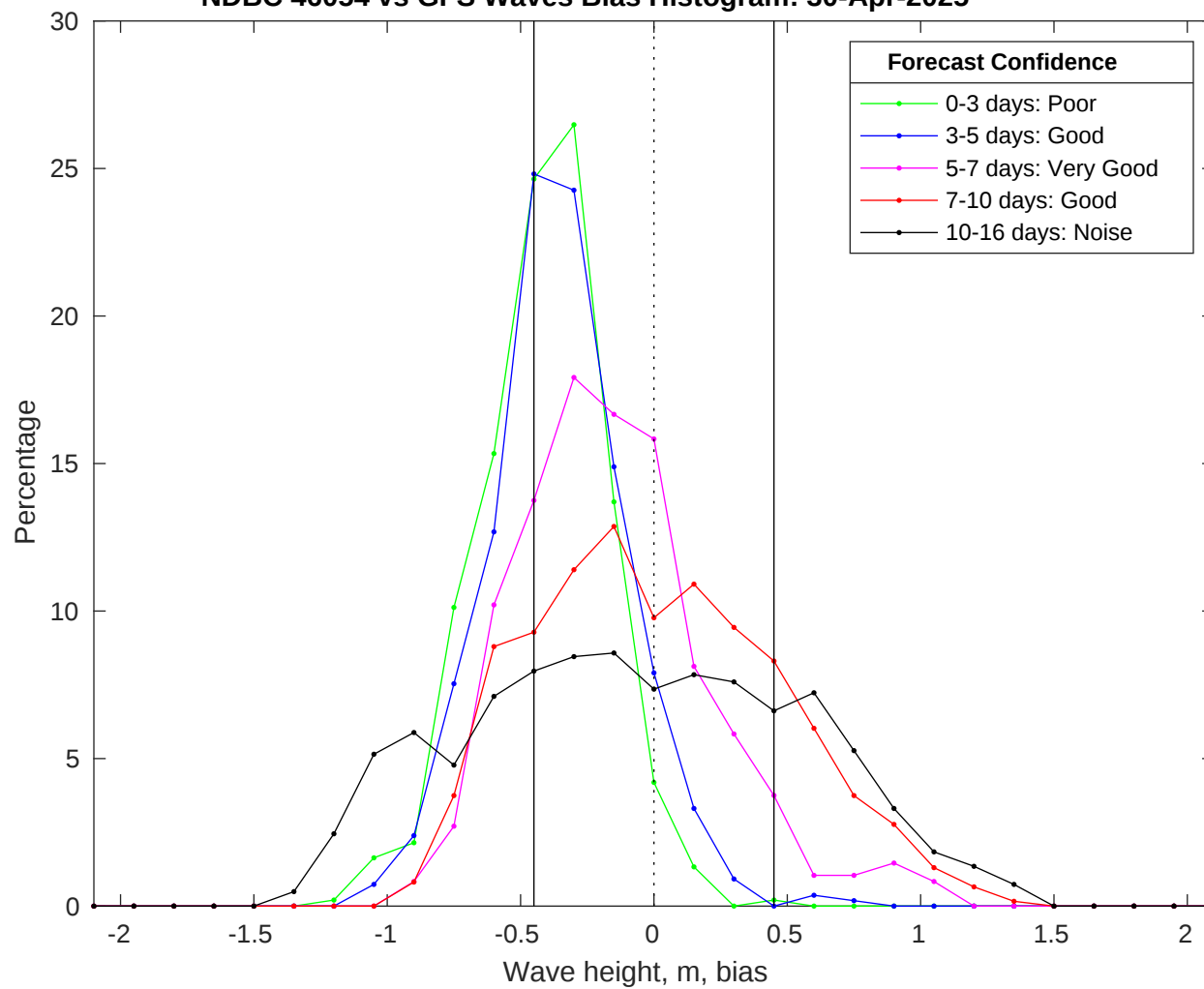
NDBC 46054 vs GFS Waves Bias Histogram: 30-Apr-2025
