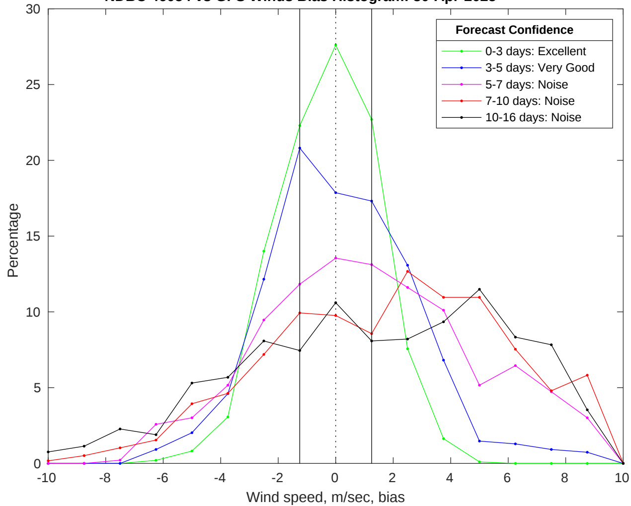
NDBC 46054 vs GFS Winds Bias Histogram: 30-Apr-2025
