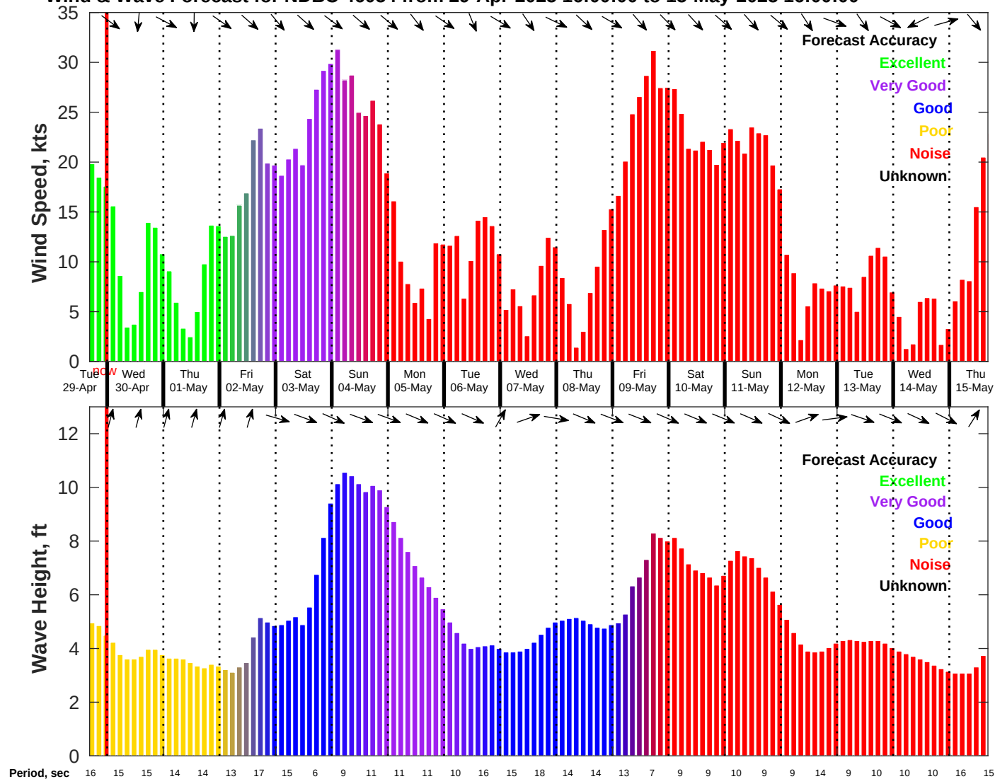
Wind & Wave Forecast for NDBC 46054 from 29-Apr-2025 16:00:00 to 15-May-2025 16:00:00
