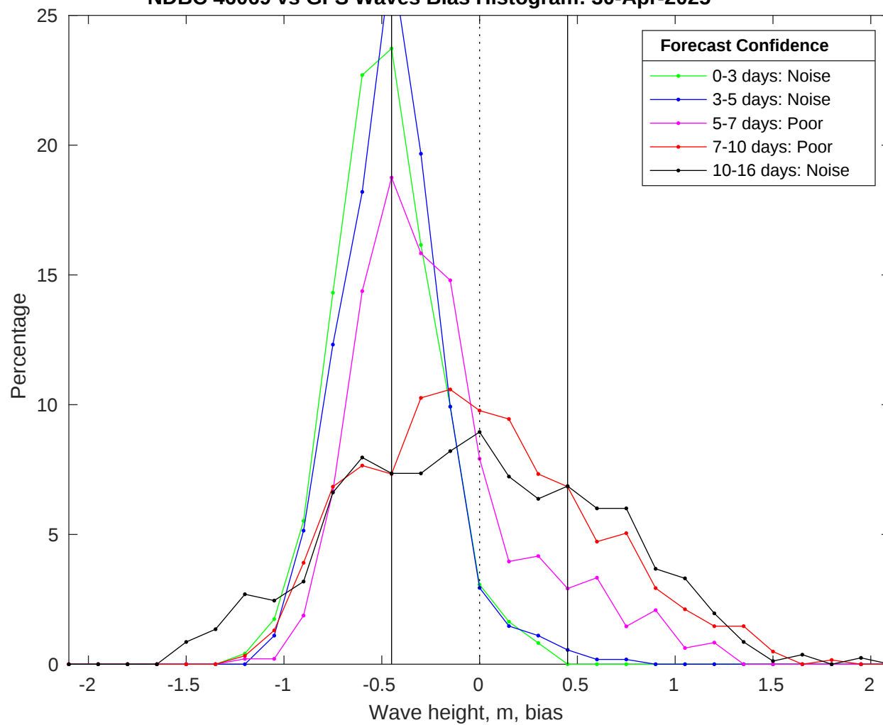
NDBC 46069 vs GFS Waves Bias Histogram: 30-Apr-2025
