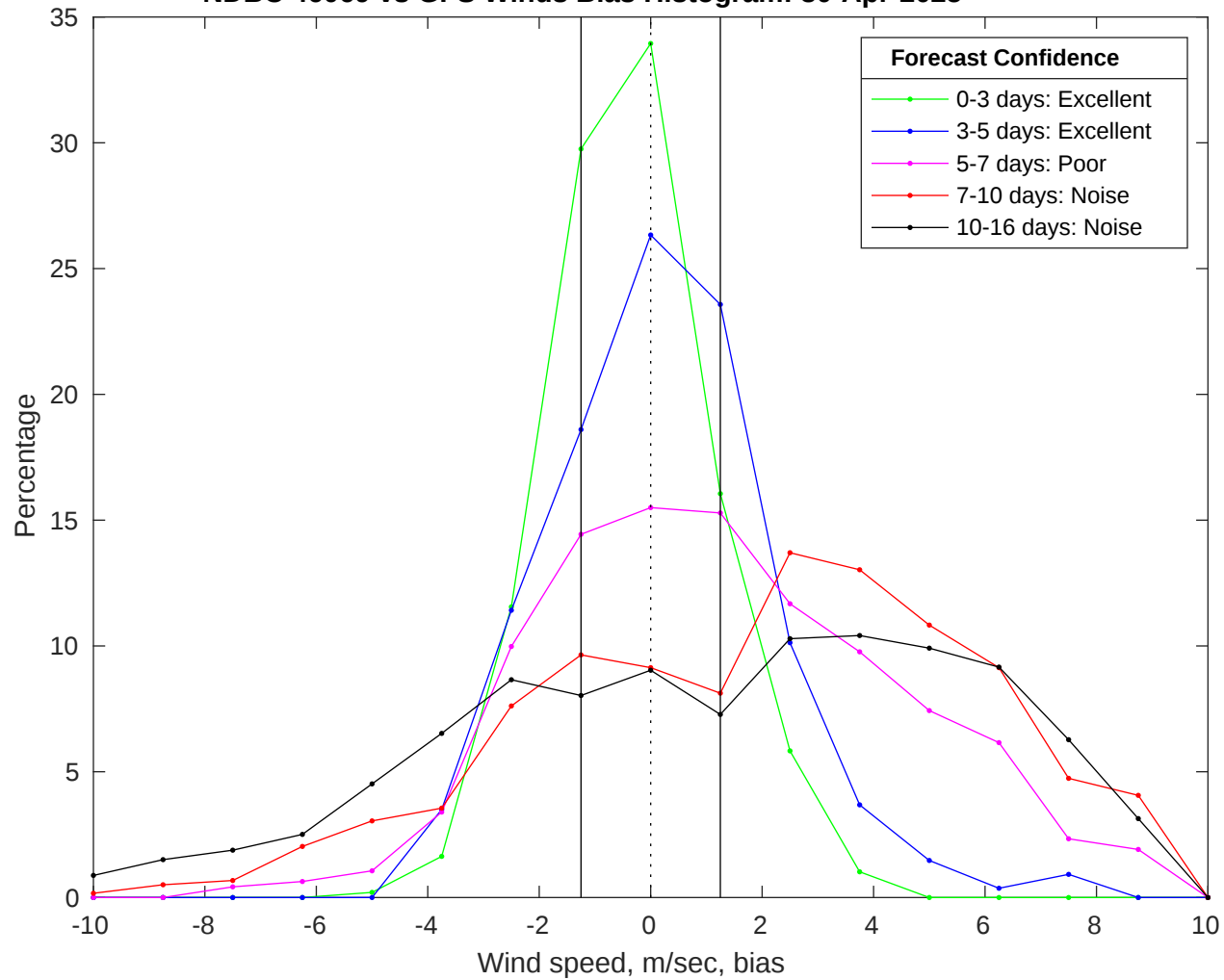
NDBC 46069 vs GFS Winds Bias Histogram: 30-Apr-2025
