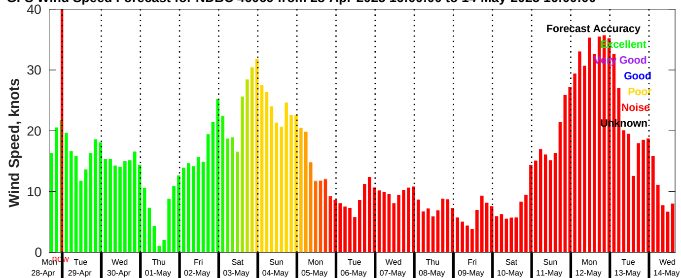
GFS Wind Speed Forecast for NDBC 46069 from 28-Apr-2025 16:00:00 to 14-May-2025 16:00:00
