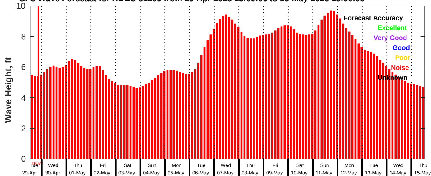
GFS Wave Forecast for NDBC 51209 from 29-Apr-2025 13:00:00 to 15-May-2025 13:00:00
