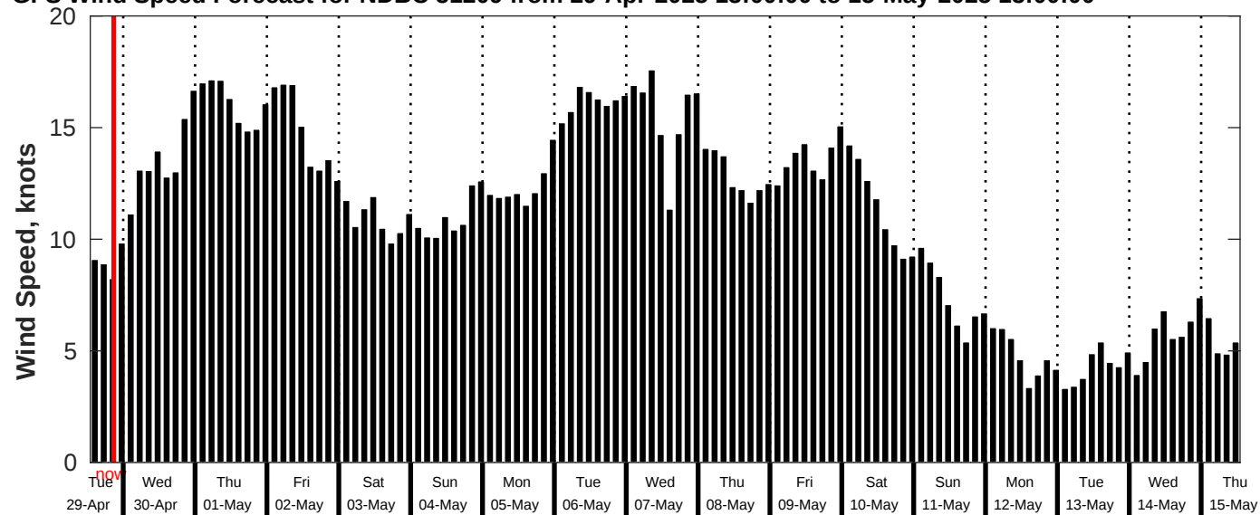
GFS Wind Speed Forecast for NDBC 51209 from 29-Apr-2025 13:00:00 to 15-May-2025 13:00:00
