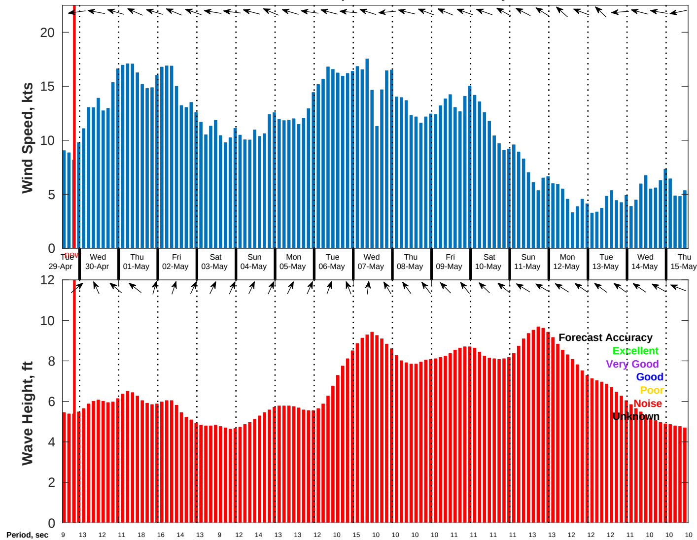
Wind & Wave Forecast for NDBC 51209 from 29-Apr-2025 13:00:00 to 15-May-2025 13:00:00
