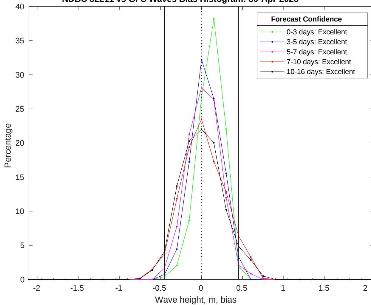
NDBC 52211 vs GFS Waves Bias Histogram: 30-Apr-2025
