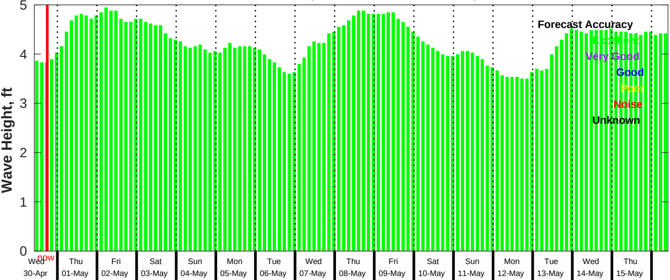
GFS Wave Forecast for NDBC 52211 from 29-Apr-2025 10:00:00 to 15-May-2025 10:00:00
