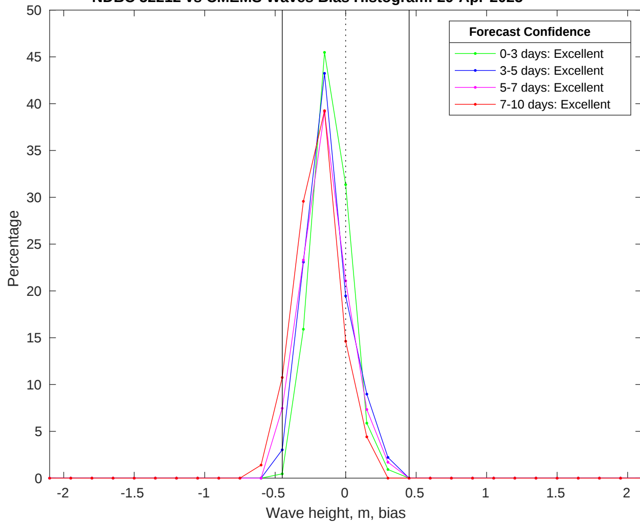
NDBC 52212 vs CMEMS Waves Bias Histogram: 29-Apr-2025
