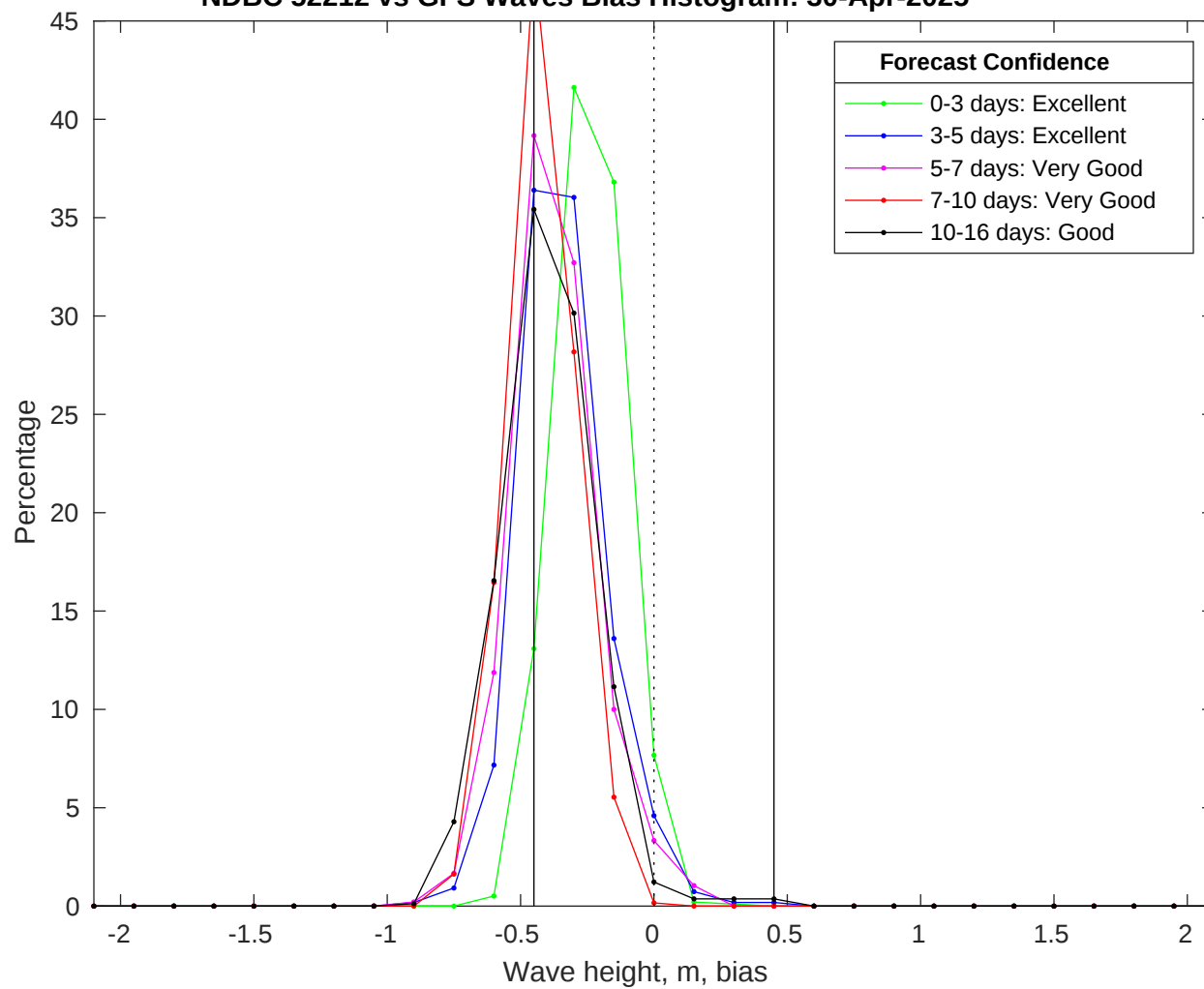
NDBC 52212 vs GFS Waves Bias Histogram: 30-Apr-2025
