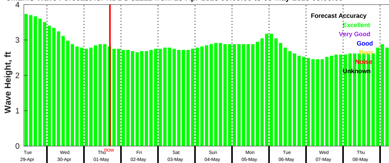
CMEMS Wave Forecast for NDBC 52212 from 28-Apr-2025 09:00:00 to 08-May-2025 09:00:00
