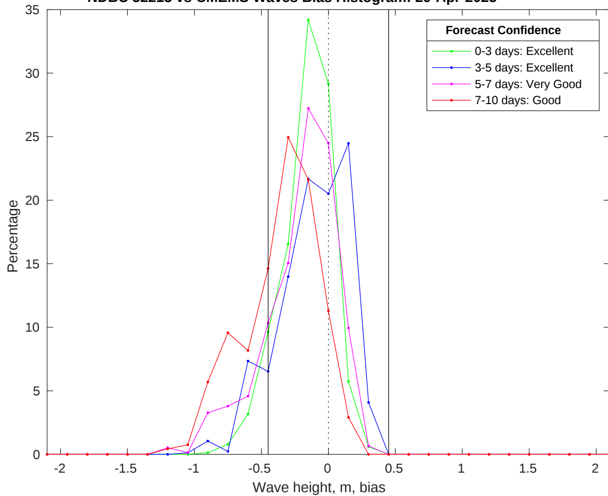
NDBC 52213 vs CMEMS Waves Bias Histogram: 29-Apr-2025
