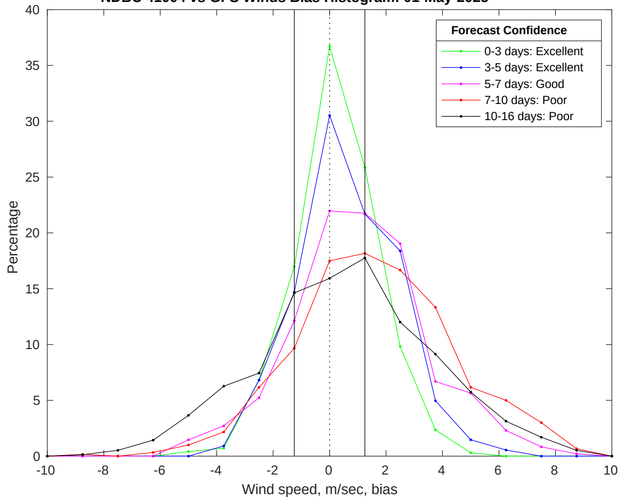
NDBC 41004 vs GFS Winds Bias Histogram: 01-May-2025
