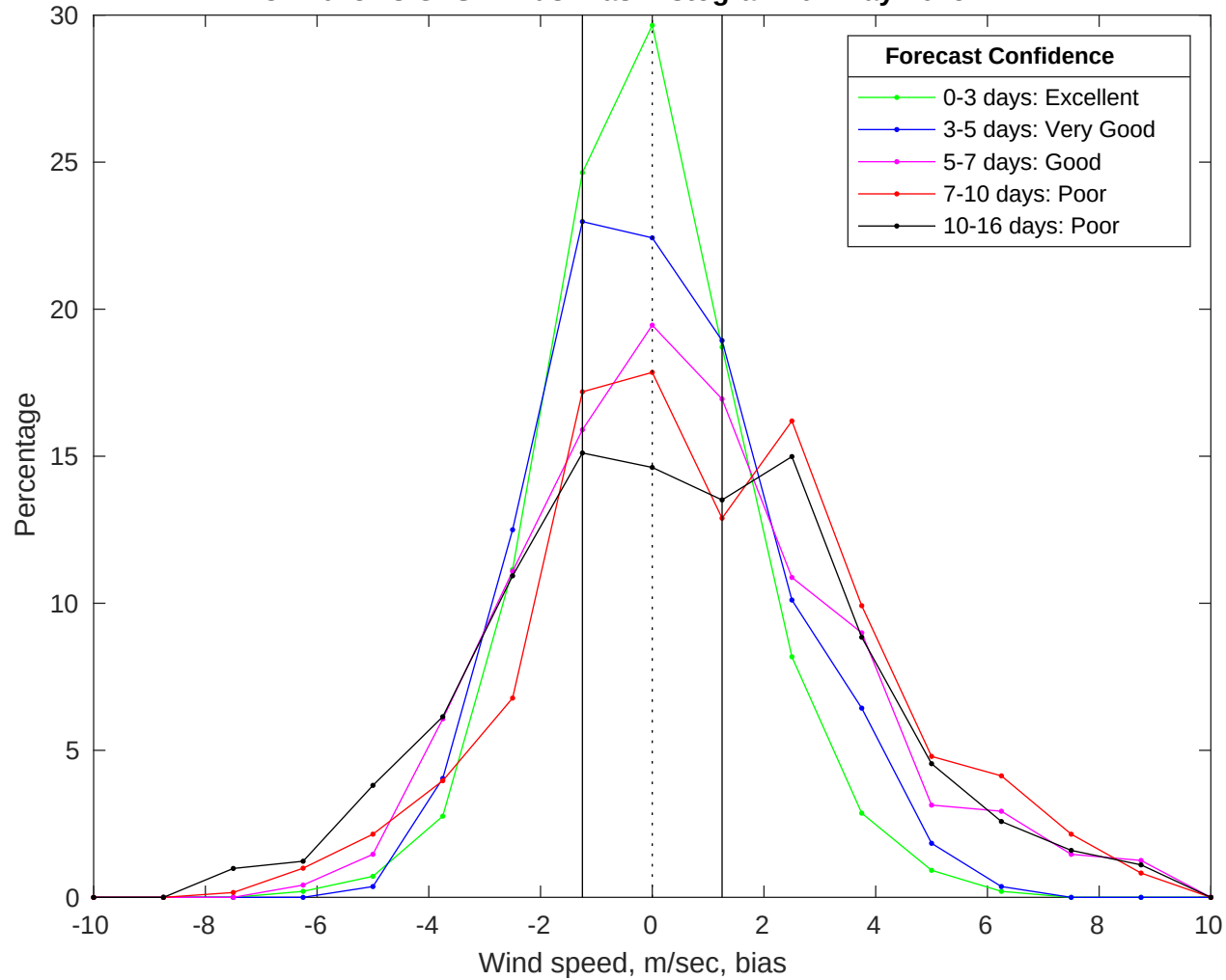
NDBC 41013 vs GFS Winds Bias Histogram: 01-May-2025
