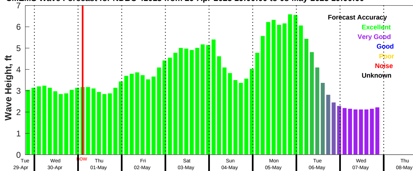
CMEMS Wave Forecast for NDBC 41013 from 29-Apr-2025 19:00:00 to 08-May-2025 19:00:00
