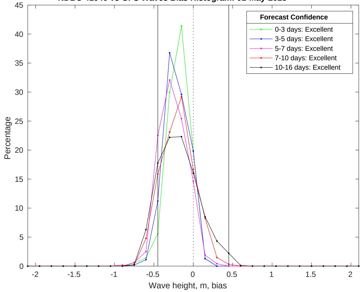
NDBC 41040 vs GFS Waves Bias Histogram: 01-May-2025
