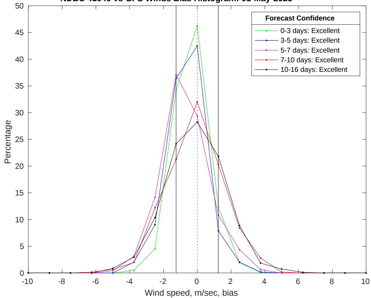
NDBC 41040 vs GFS Winds Bias Histogram: 01-May-2025
