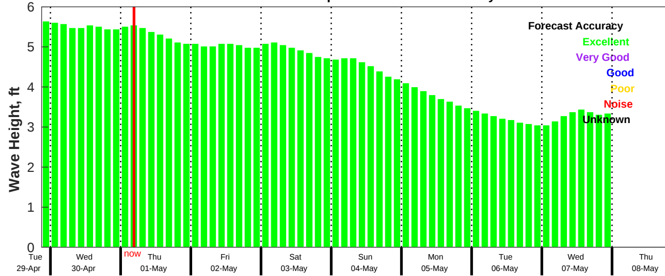
CMEMS Wave Forecast for NDBC 41040 from 29-Apr-2025 21:00:00 to 08-May-2025 21:00:00
