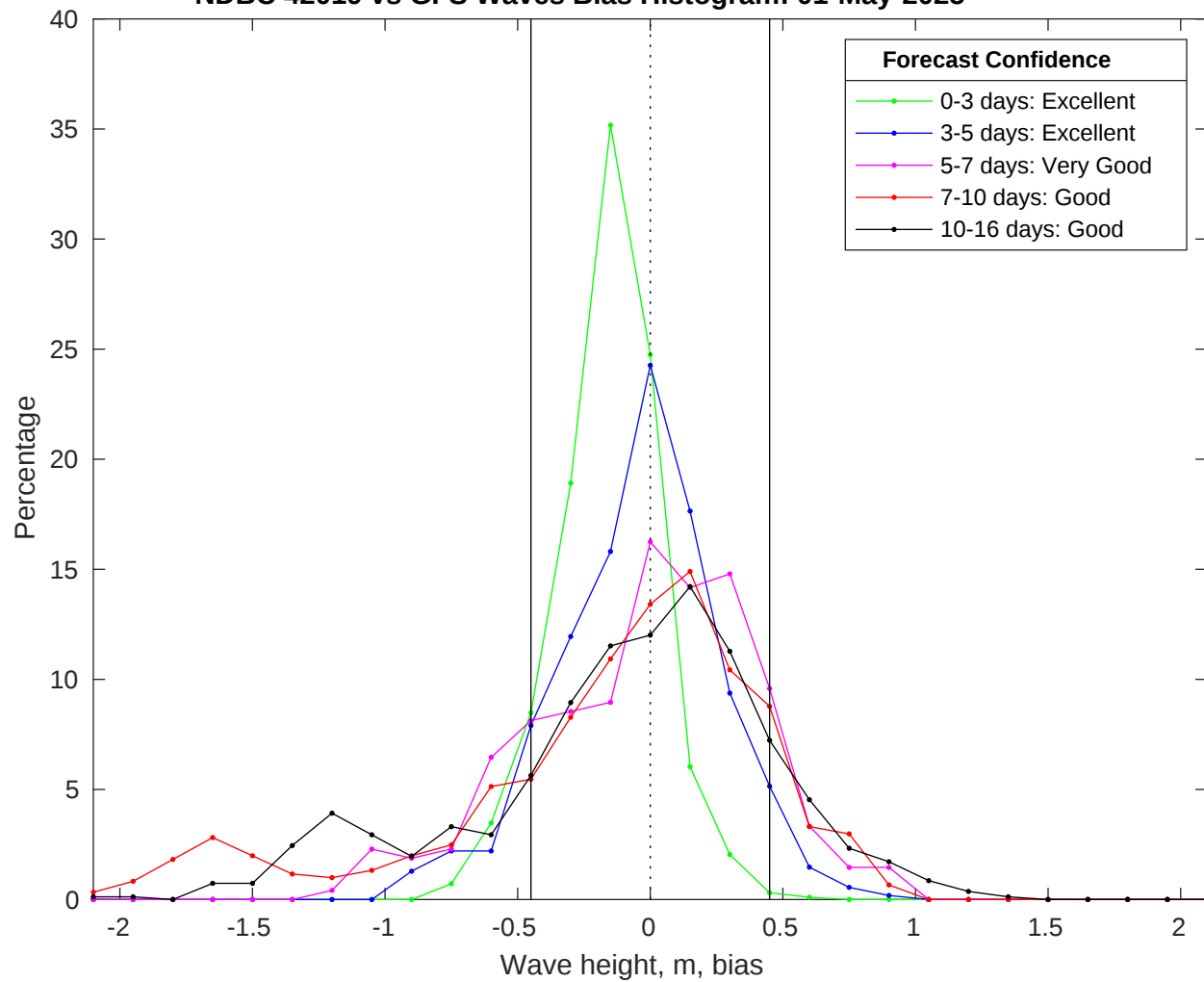
NDBC 42019 vs GFS Waves Bias Histogram: 01-May-2025
