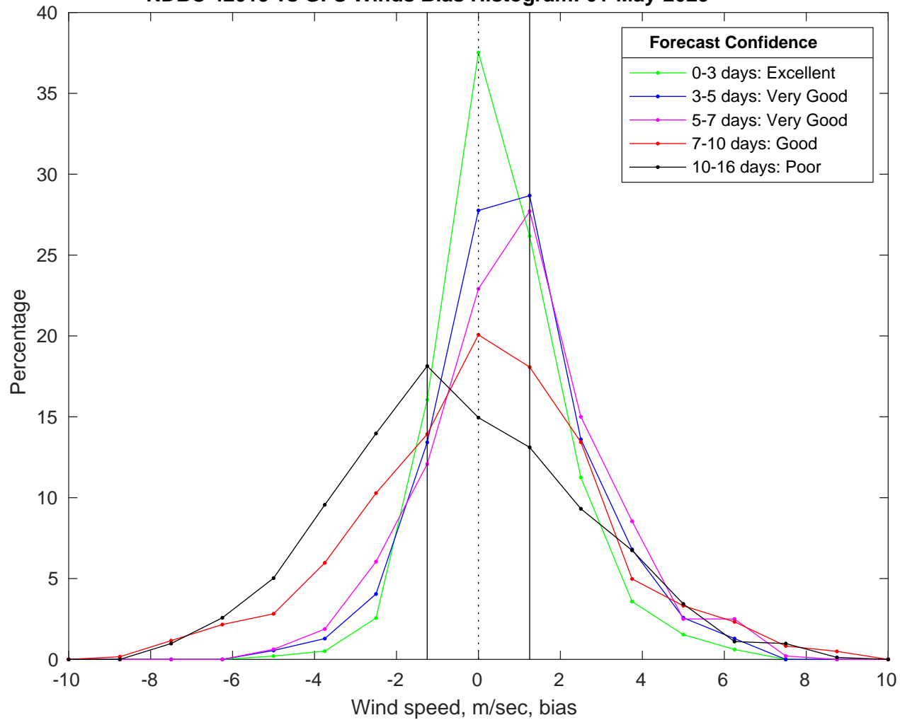
NDBC 42019 vs GFS Winds Bias Histogram: 01-May-2025
