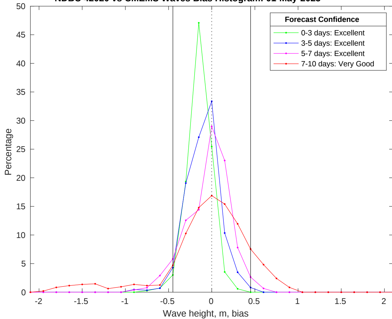
NDBC 42020 vs CMEMS Waves Bias Histogram: 01-May-2025
