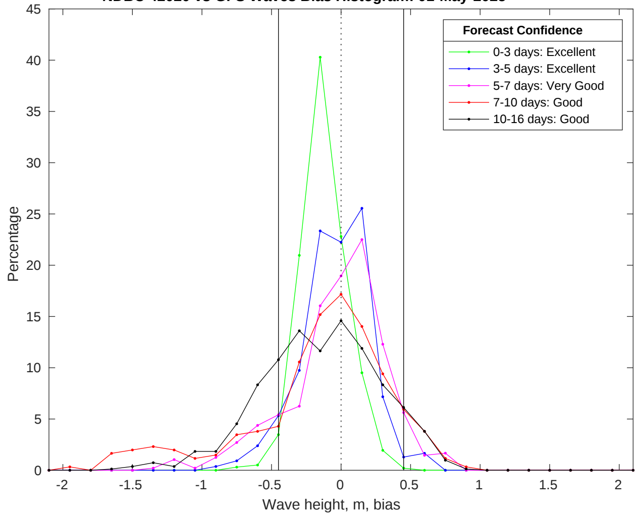
NDBC 42020 vs GFS Waves Bias Histogram: 01-May-2025
