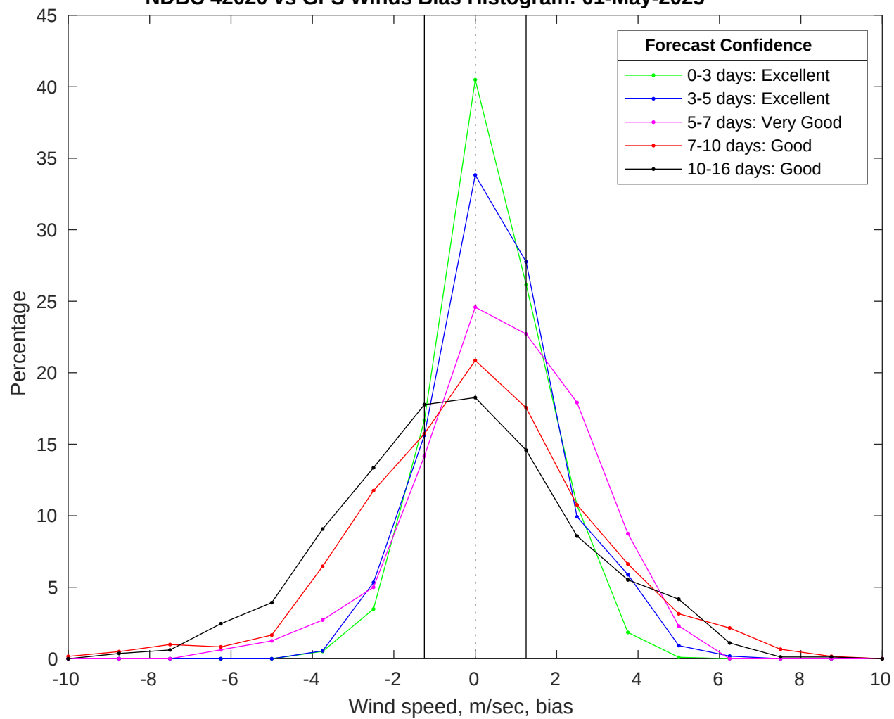
NDBC 42020 vs GFS Winds Bias Histogram: 01-May-2025
