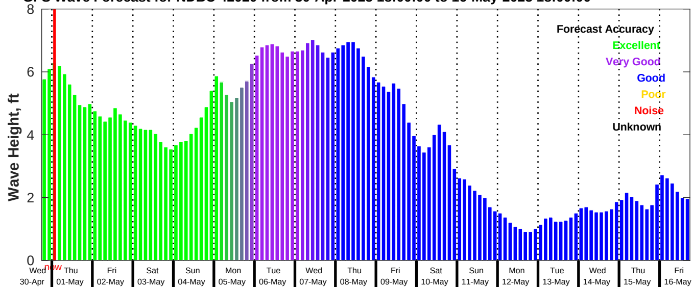
GFS Wave Forecast for NDBC 42020 from 30-Apr-2025 18:00:00 to 16-May-2025 18:00:00
