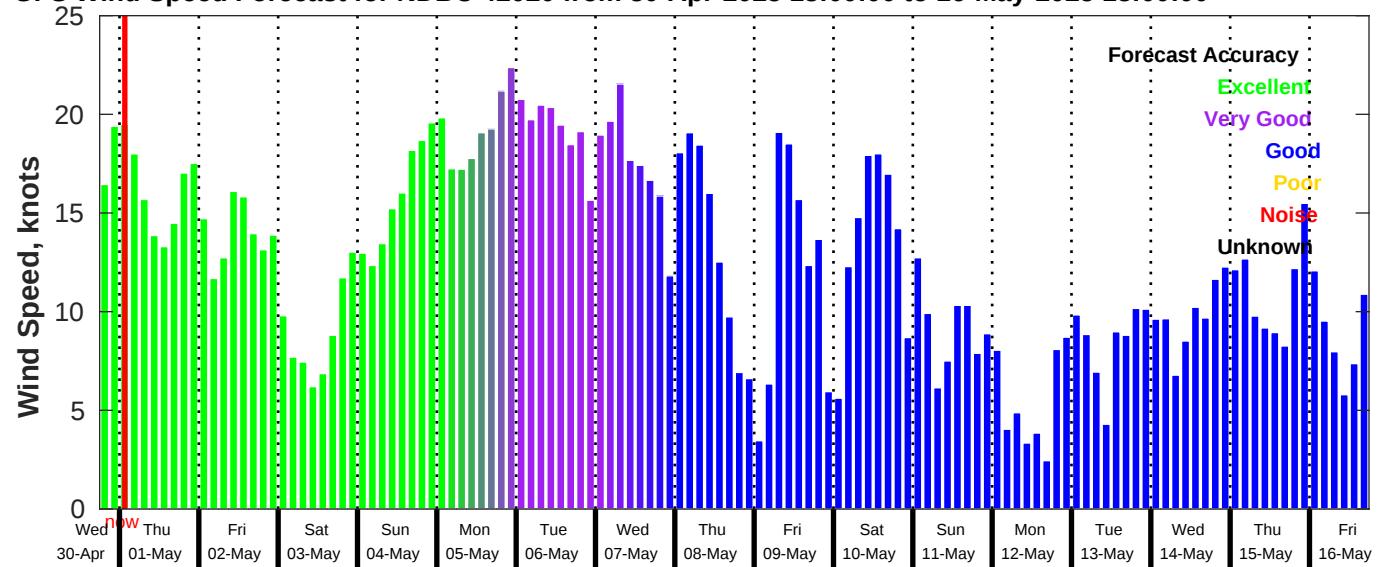
GFS Wind Speed Forecast for NDBC 42020 from 30-Apr-2025 18:00:00 to 16-May-2025 18:00:00
