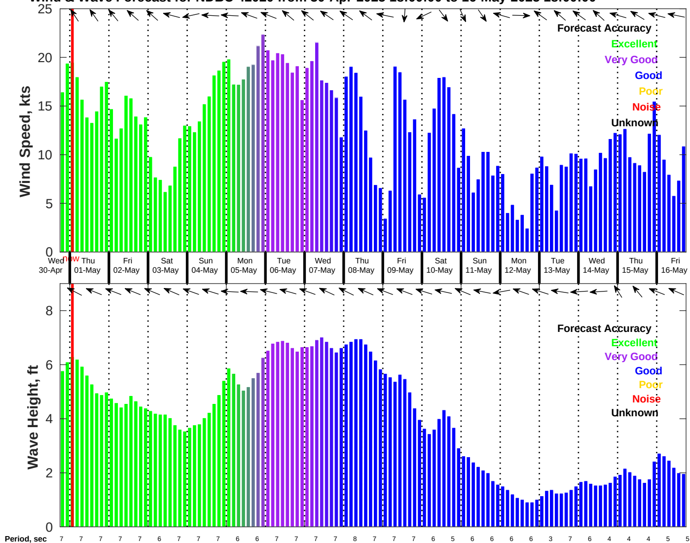
Wind & Wave Forecast for NDBC 42020 from 30-Apr-2025 18:00:00 to 16-May-2025 18:00:00
