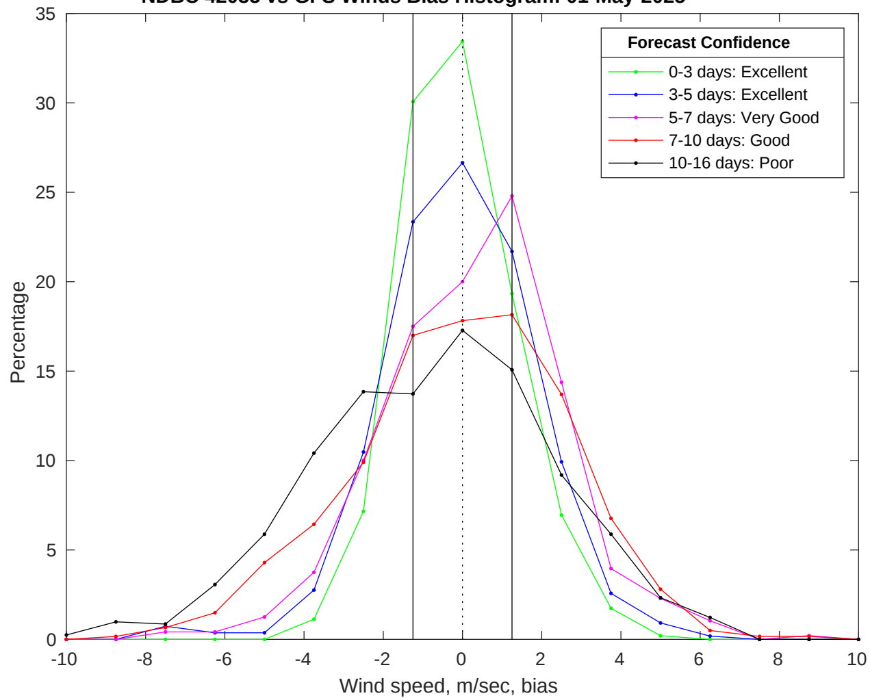
NDBC 42035 vs GFS Winds Bias Histogram: 01-May-2025
