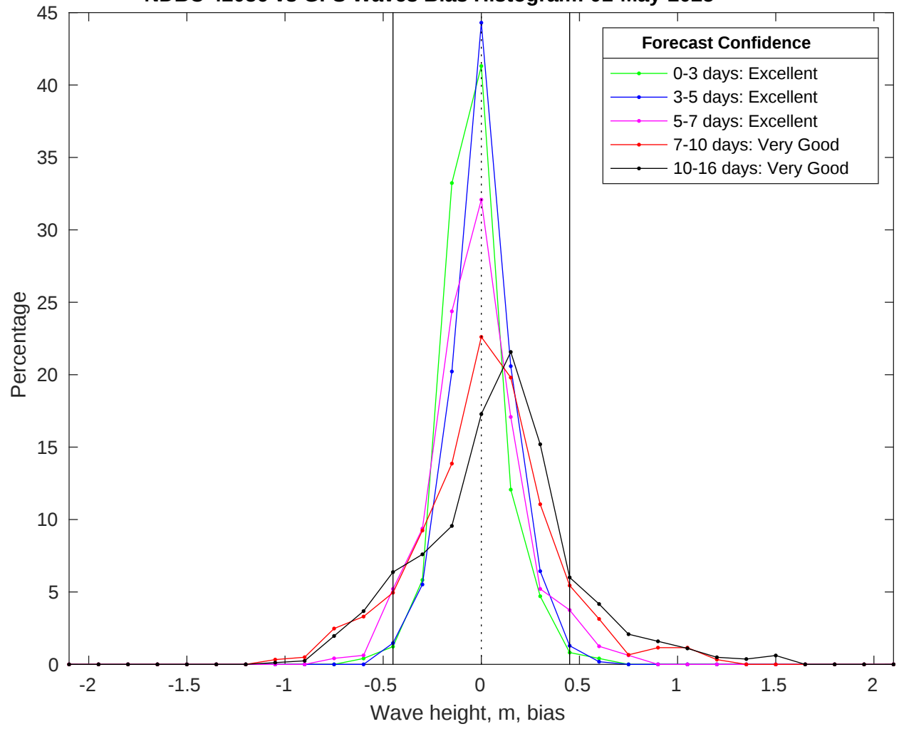
NDBC 42036 vs GFS Waves Bias Histogram: 01-May-2025
