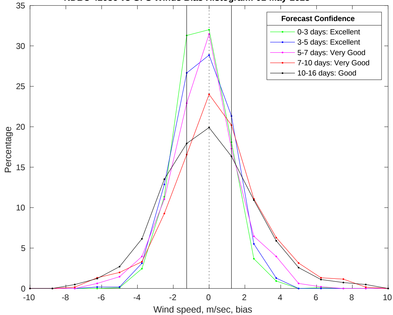
NDBC 42036 vs GFS Winds Bias Histogram: 01-May-2025
