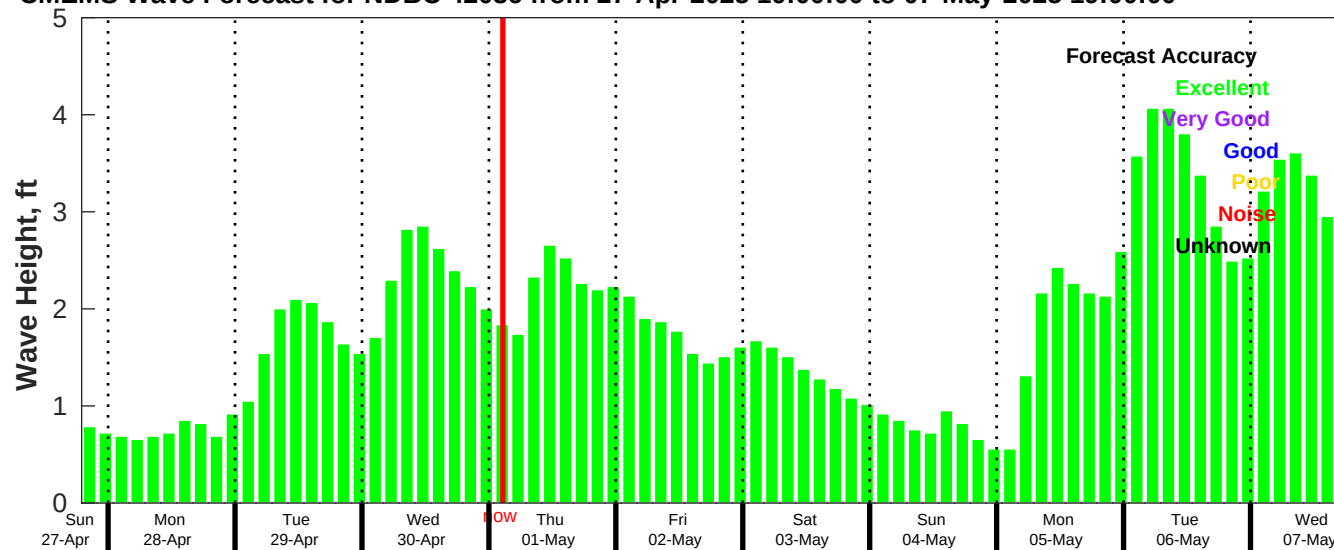
CMEMS Wave Forecast for NDBC 42036 from 27-Apr-2025 19:00:00 to 07-May-2025 19:00:00
