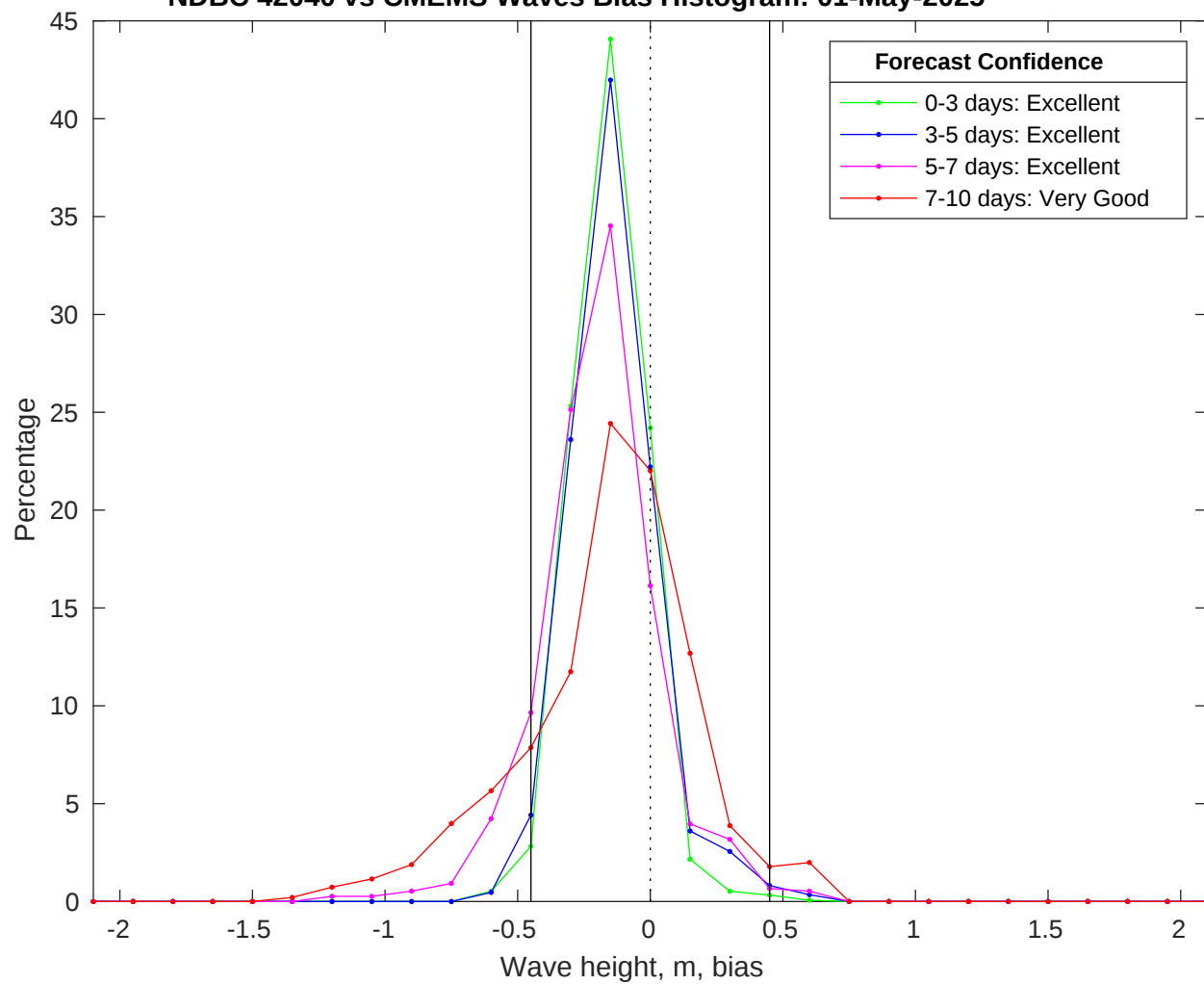
NDBC 42040 vs CMEMS Waves Bias Histogram: 01-May-2025
