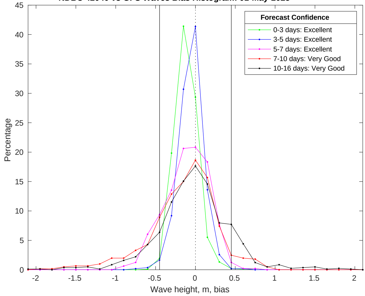
NDBC 42040 vs GFS Waves Bias Histogram: 01-May-2025
