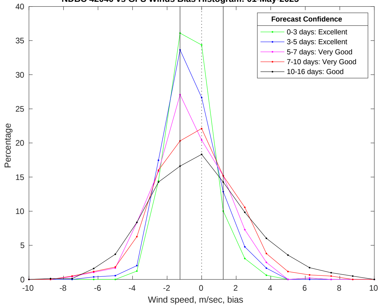
NDBC 42040 vs GFS Winds Bias Histogram: 01-May-2025
